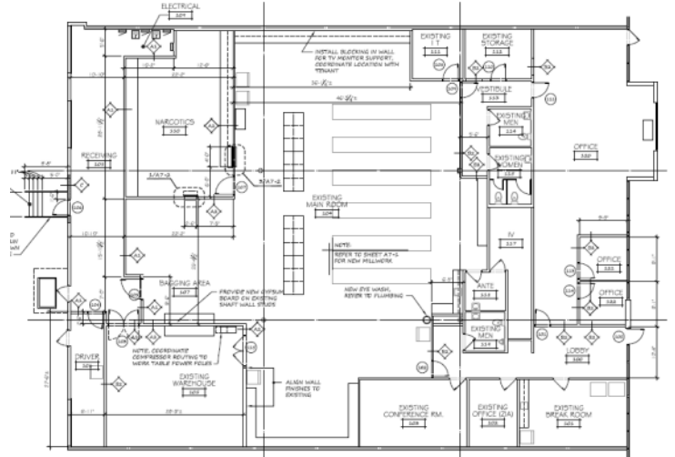
Proposed office/warehouse floor plan
